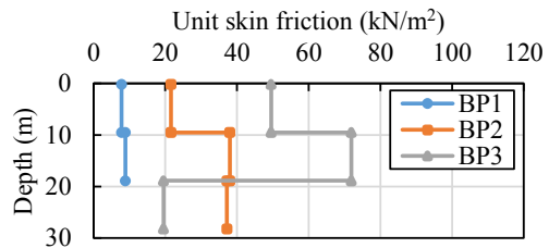
Fig. 9 Unit skin friction of each test.
