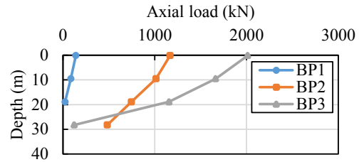
Fig. 8 Comparison of axial load of each test.
