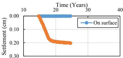
Fig. 7 Settlement during third pile load test.
