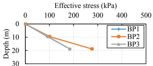
Fig. 10 Effective stress of each test.
