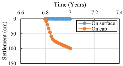
Fig. 5 Settlement during first pile load test.
