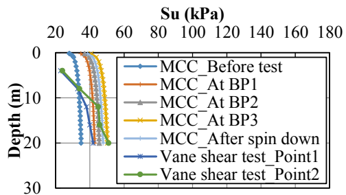
Fig. 12 Comparison of undrained shear strength.
