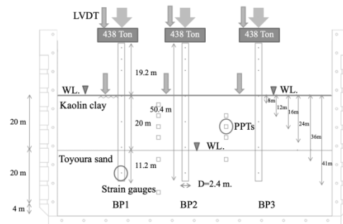
Fig. 4 Testing procedure of centrifuge tests.
