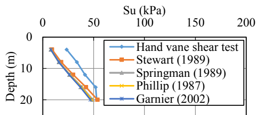
Fig. 11 Comparison of undrained shear strength.
