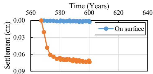
Fig. 6 Settlement during second pile load test.
