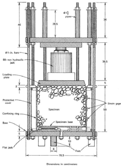
(a) Fixed ring (Marsal, 1973)
