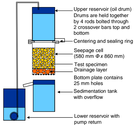
Figure 2 Permeameter cell (Kenney and Lau, 1985)
