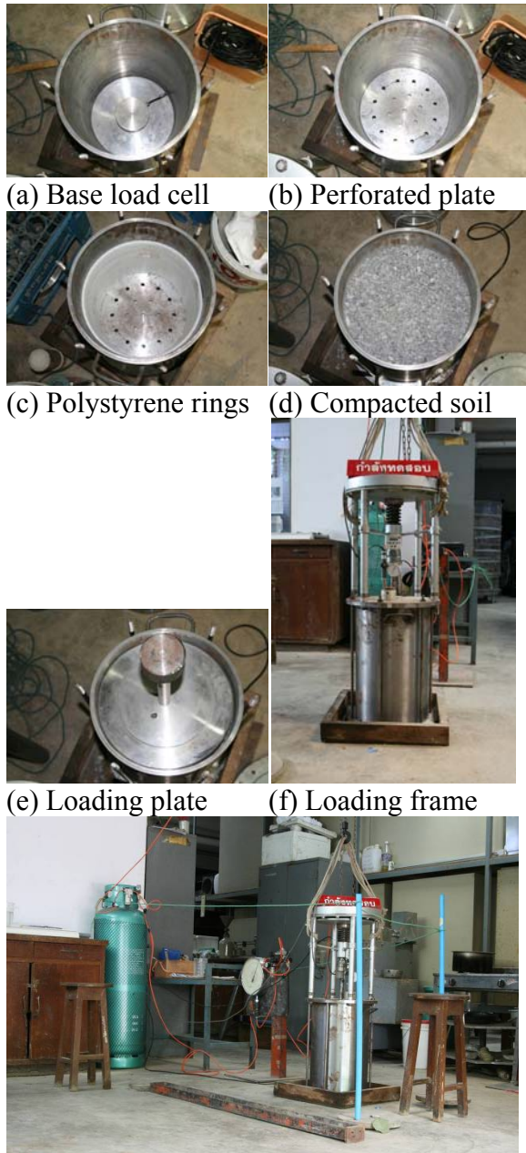
(g) Full assembly in dry condition Figure 5 Device assembly
