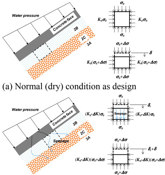
(b) Seepage through condition Figure 8 Testing conditions of cushion layer
