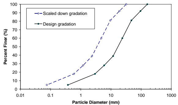
Figure 7 Grain size distributions of cushion layer and specimen
